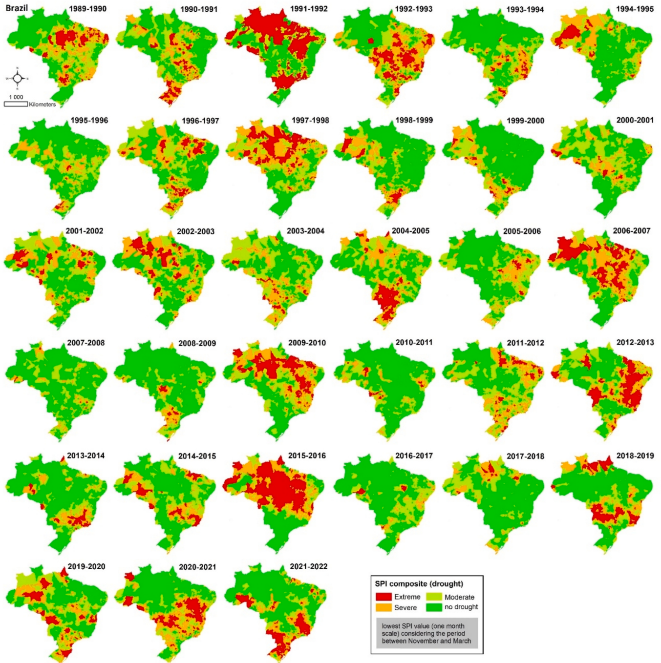
Fig. 2. Spatiotemporal drought occurrence (according to the SPI composite) across Brazil during the growing seasons of 1990 to 2022.
